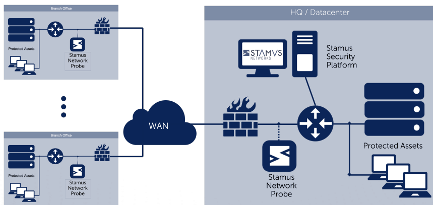
Figure 2. Stamus ND/NDR – independent probe management and threat hunting systems may access multiple probes in multiple branch offices or network segments.
