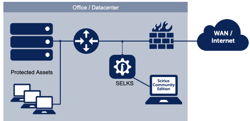
Figure 1. SELKS - a single instance of Suricata with the management system integrated into the sensor.
